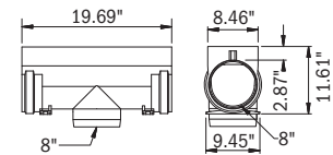
HydroBlock 200 - Bottom Outlet Section Grate Free-Area: Std = 60 in 2 | ADA = 43 in 2
