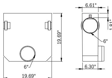
HydroBlock™ 150 Grate Free-Area: Std = 40 in 2 | ADA = 29 in 2
