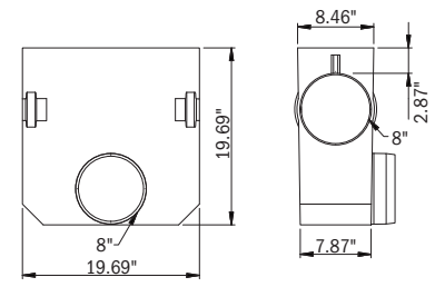
HydroBlock™ 200 Grate Free-Area: Std = 60 in 2 | ADA = 43 in 2
