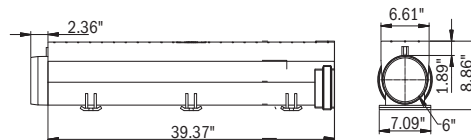
HydroBlock 150 Grate Free-Area: Std = 80 in 2 /m | ADA = 59 in 2 /m
