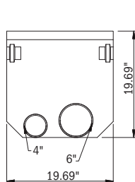
HydroBlock™ 100 Grate Free-Area: 26 in 2
