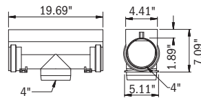
HydroBlock 100 - Bottom Outlet Section Grate Free-Area: 26 in 2
