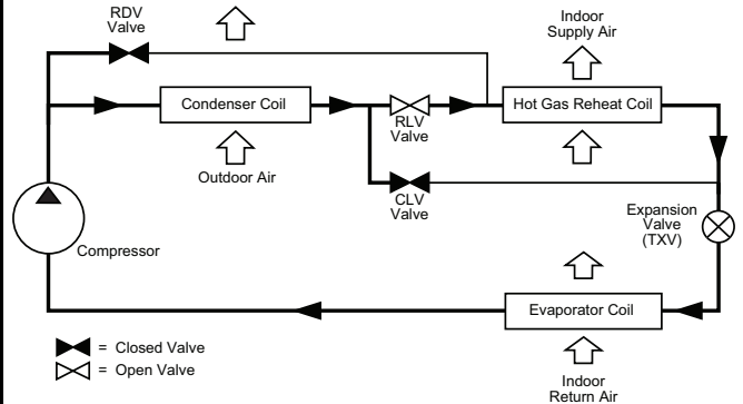
Subcooling Mode (Reheat1) — Hot Gas Re-Heat System with 2-Stage Cooling
