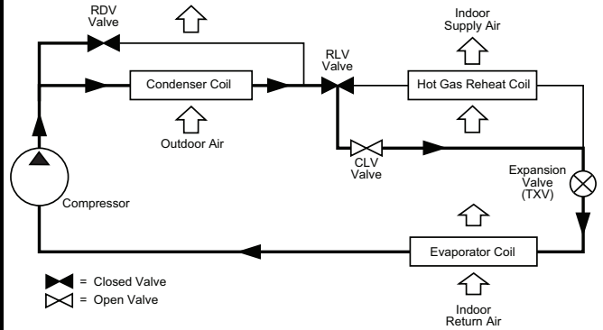
Normal Cooling Mode — Hot Gas Re-Heat System with 2-Stage Cooling
