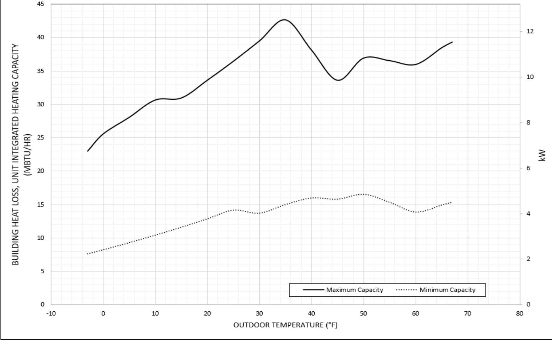
3 TON BALANCE POINT WORKSHEET COMFORT MINIMUM AND MAXIMUM HEATING CAPACITIES
