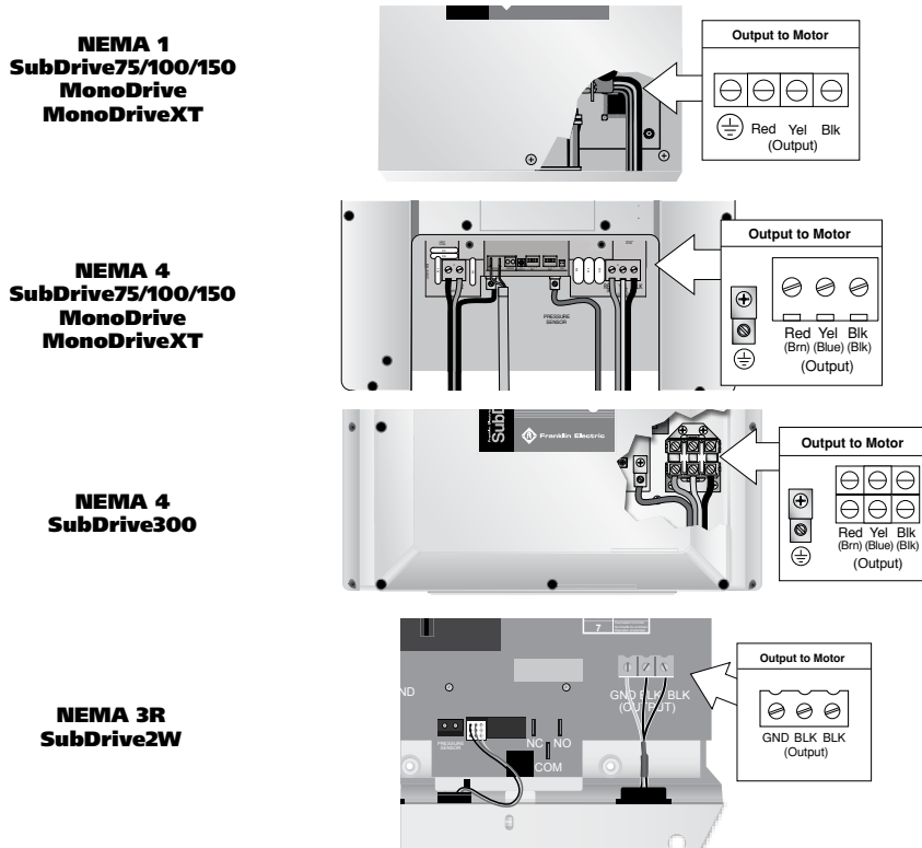
Figure 3: Motor Lead Connections
