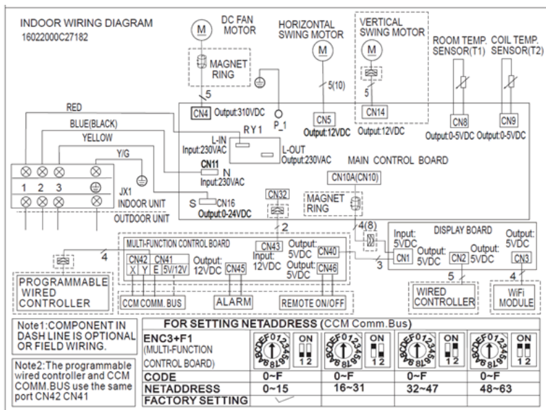
Fig. 18 — Wiring Diagram 18K-24K
