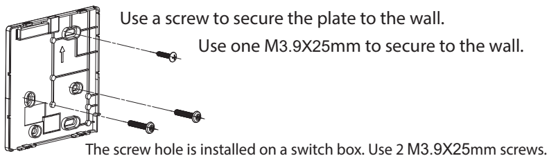
Fig. 5 — Screw to wall
