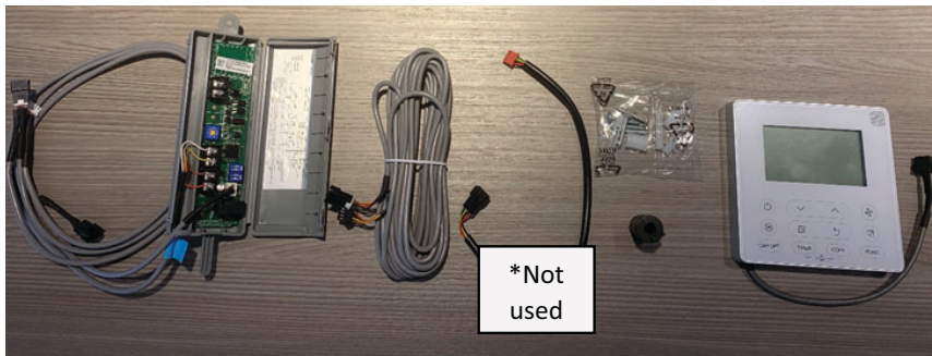
Fig. 10 — Identify the components
