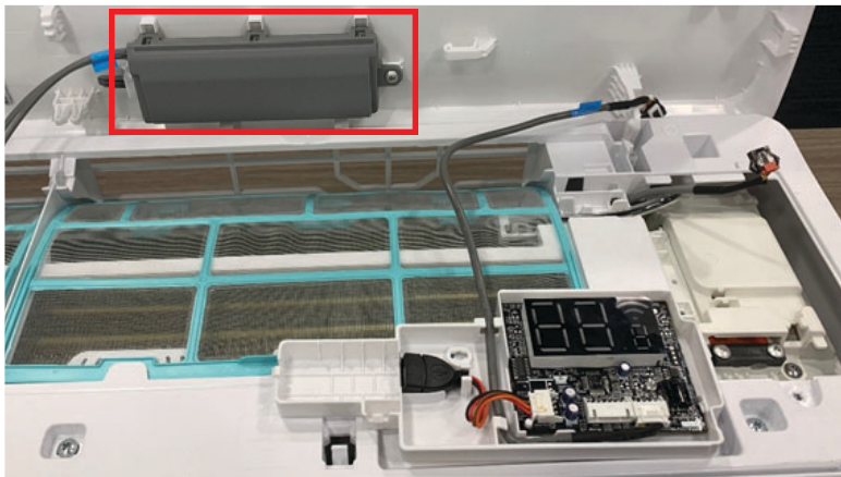
Fig. 14 — Insert and screw the adapter board into place
