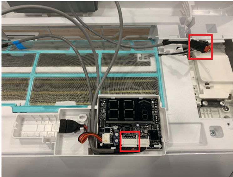
Fig. 15 — Install the white 7-pin plug
