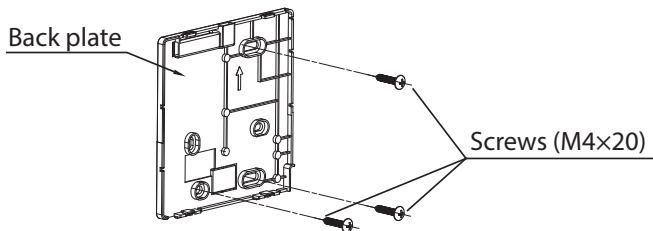
Fig. 4 — Back plate
