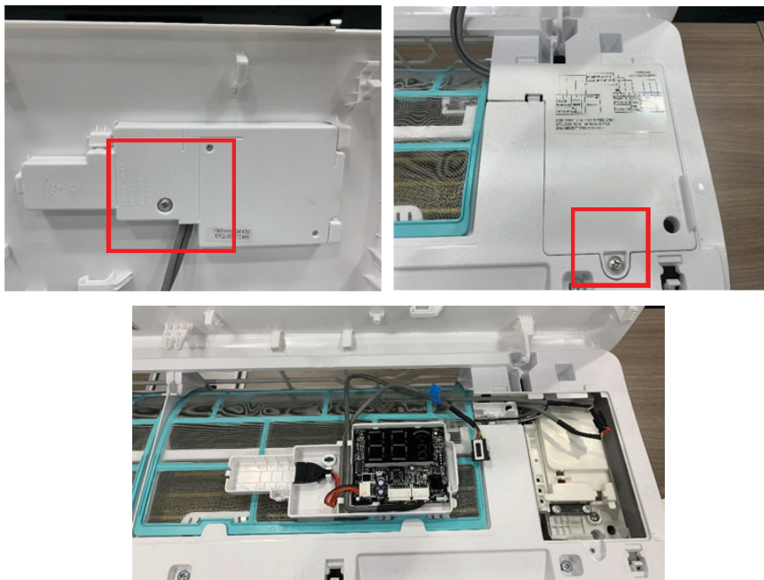
Fig. 12 — Open the terminal block and display board covers
