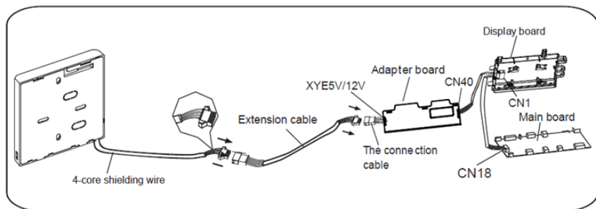
Fig. 9 — Installation of KSACN0901AAA
