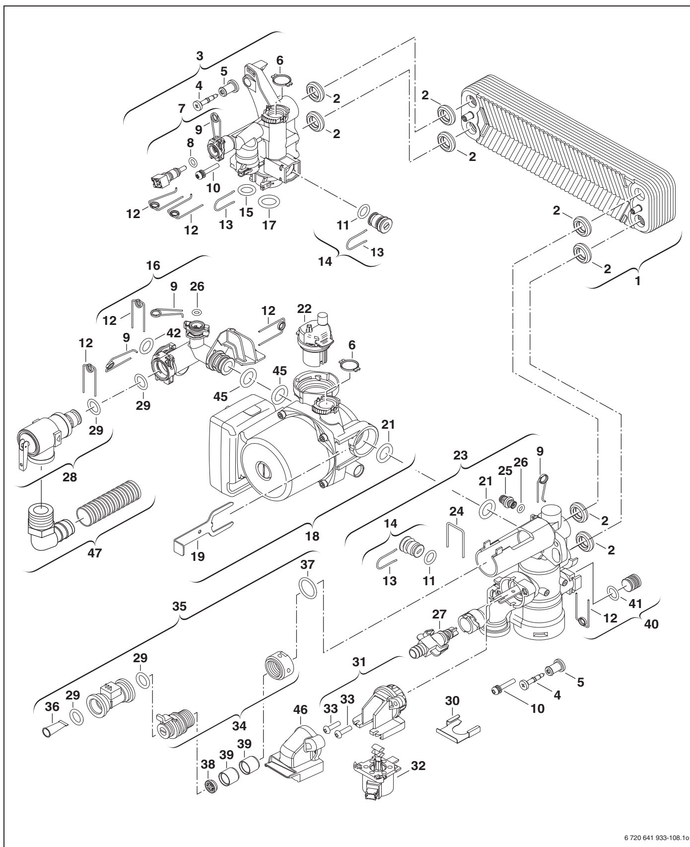
Fig. 99 Group 7 - Hydraulic block combi boiler ZWB.-3A Greenstar
