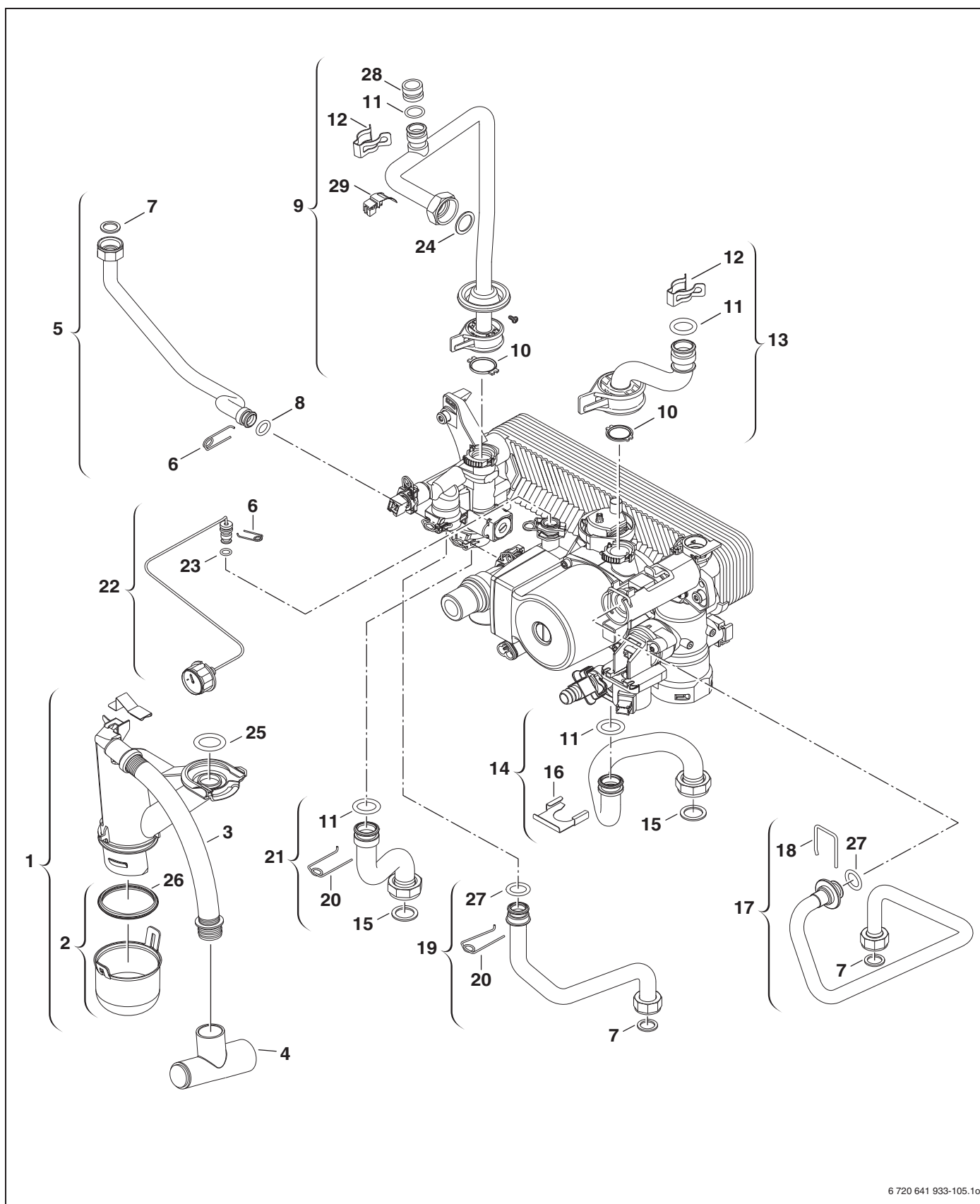
Fig. 96 Group 4 - Pipes combi boiler ZWB.-3A Greenstar
