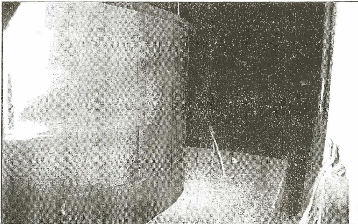
PHOTO 2: Static Load @ 3,1950 LBS on HDPE Adjusting Ring configuration 2 @ 2'' and 3 @ 4''
