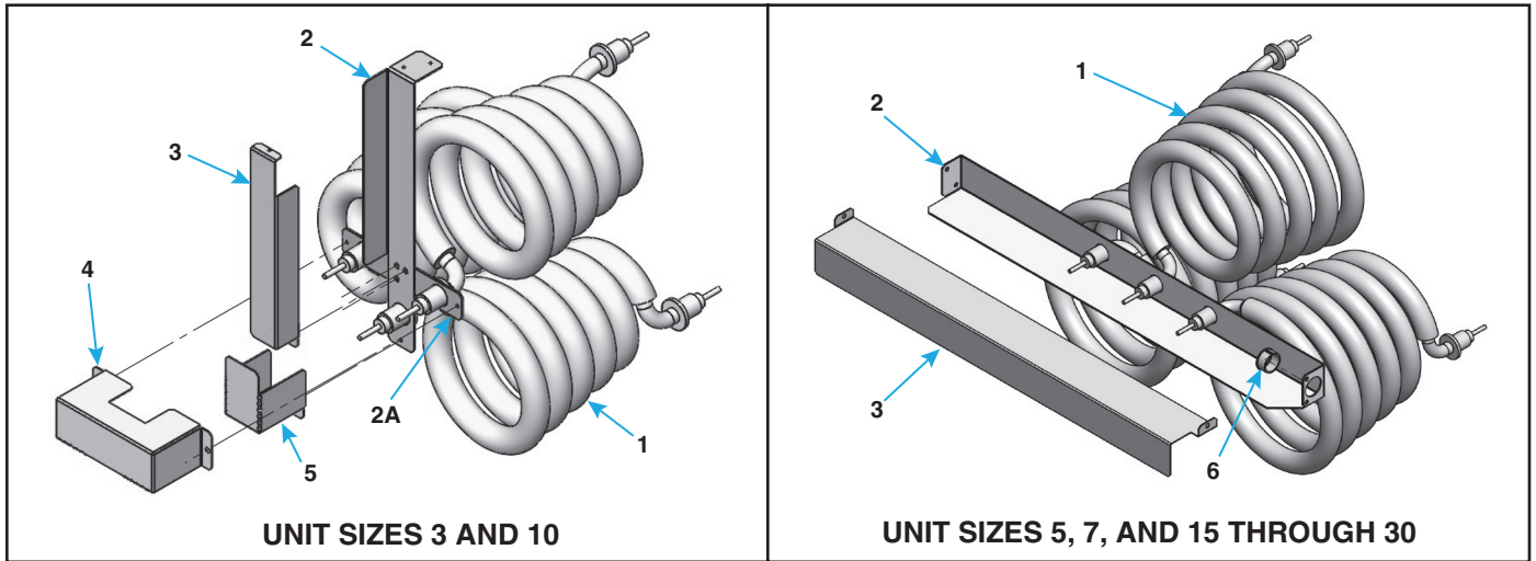
Figure 1. Typical Heating Element Assemblies (Refer to Table 3 )
