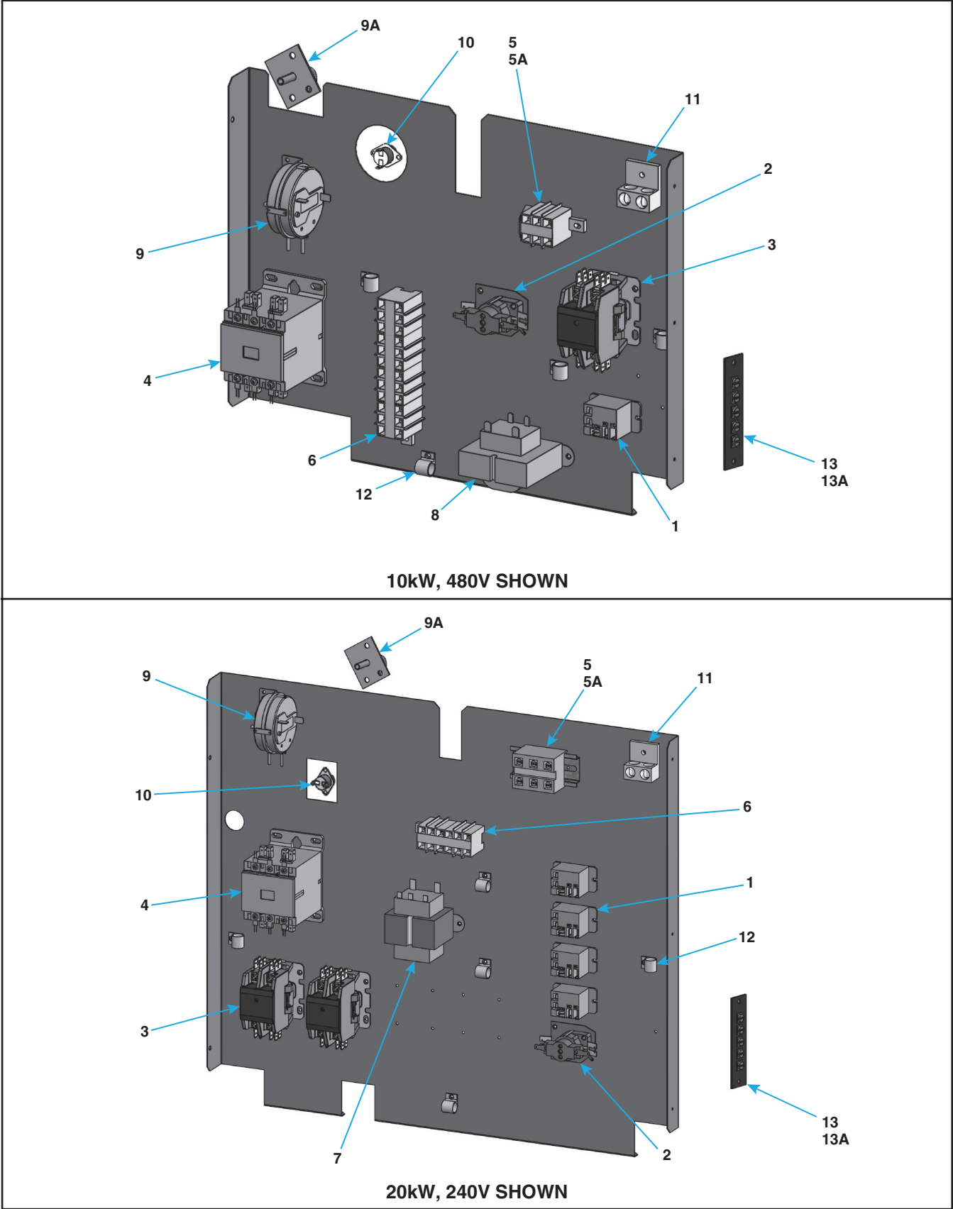
Figure 2. Typical Control Panels (Refer to Table 4 )
