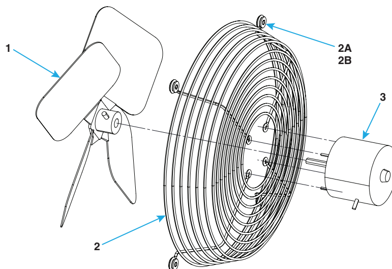
Figure 3. Fan and Motor Assembly (Refer to Table 5 )
