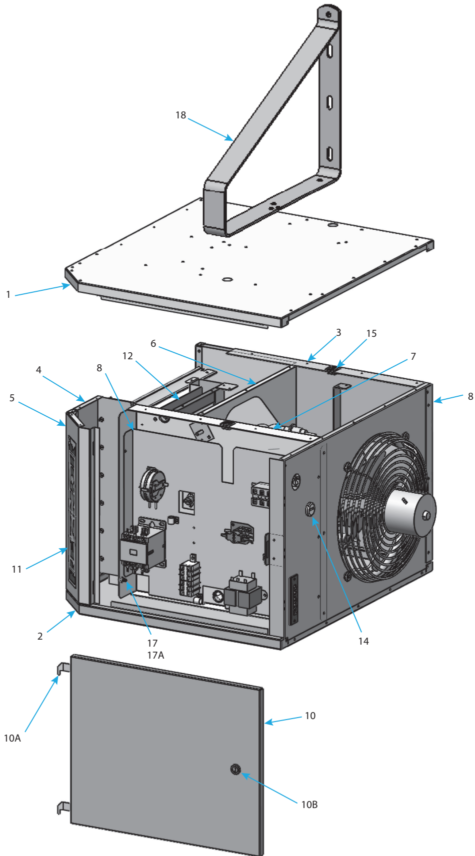
Figure 4. Cabinet Components (Refer to Table 6 )
