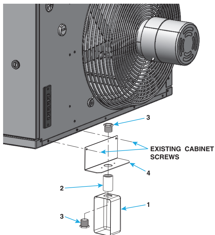
Figure 8. Thermostat Bracket Kit (Refer to Table 10 )
