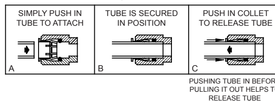
Figure 12 – Quick Connect Fittings
