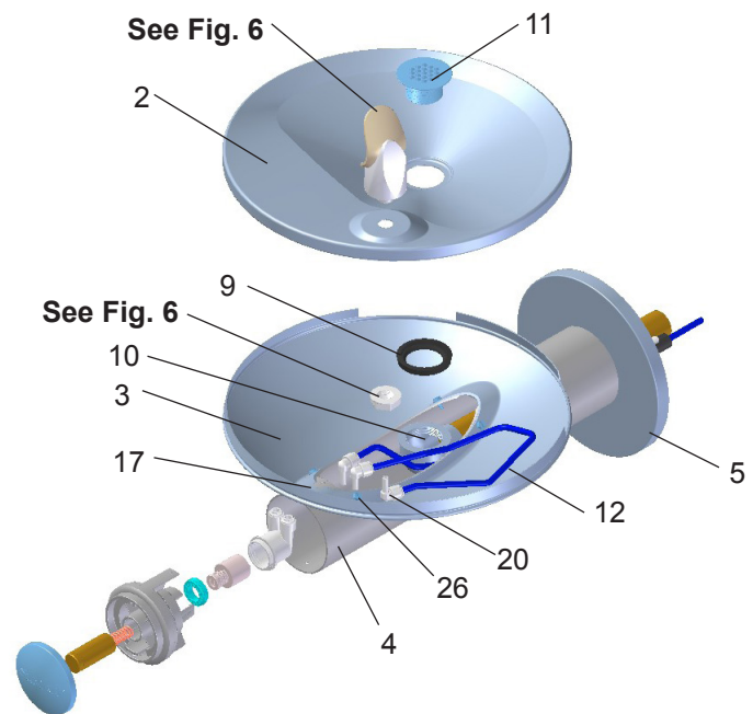
Figure 8 - Fountain Body Assembly
