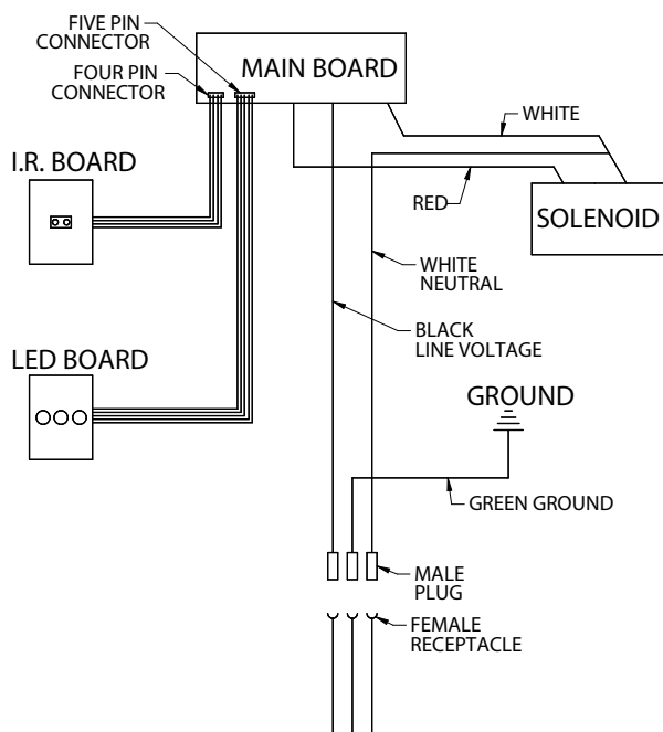
Electrical Diagram
