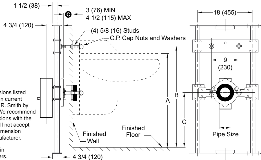
Fig. 0925Y . . . WITH SUPPORTING STUDS, ADJUSTABLE COUPLING AND WASTE FITTING 4" (100) NO-HUB AND 4" (100) VENT FOR BACK OUTLET FLUSHING RIM SERVICE SINK
