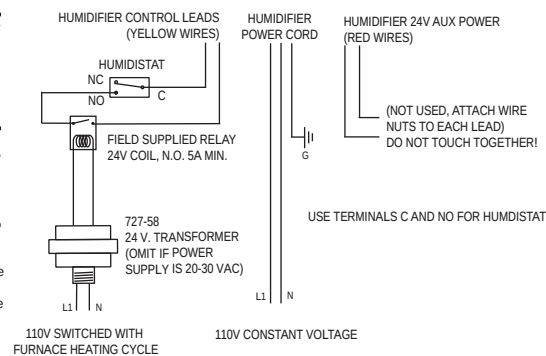
DIAGRAM 4 WIRING 120V. 1137/1000 POWER HUMIDIFIER
