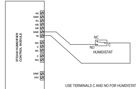
DIAGRAM 2 WIRING HIGH LIMIT HUMIDISTAT WITH ELITE STEAM HUMIDIFIER
