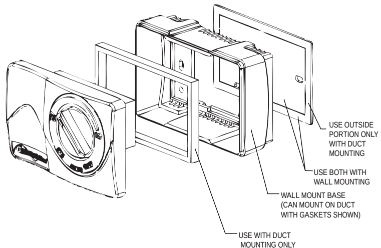
FIG. 3 GASKET PLACEMENT
