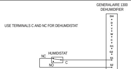
DIAGRAM 5 1300 DEHUMIDIFIER
