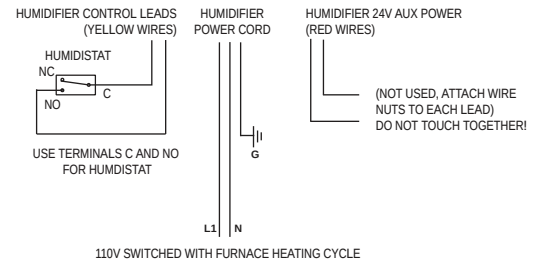
DIAGRAM 3 WIRING 120V. 1137/1000 POWER HUMIDIFIER
