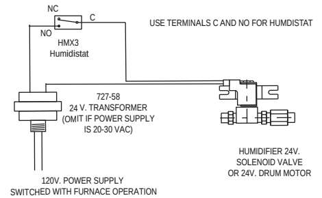
DIAGRAM 1 WIRING 24V. BYPASS HUMIDIFIER
