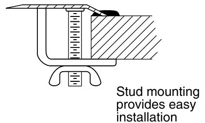
Drop-in Installation
