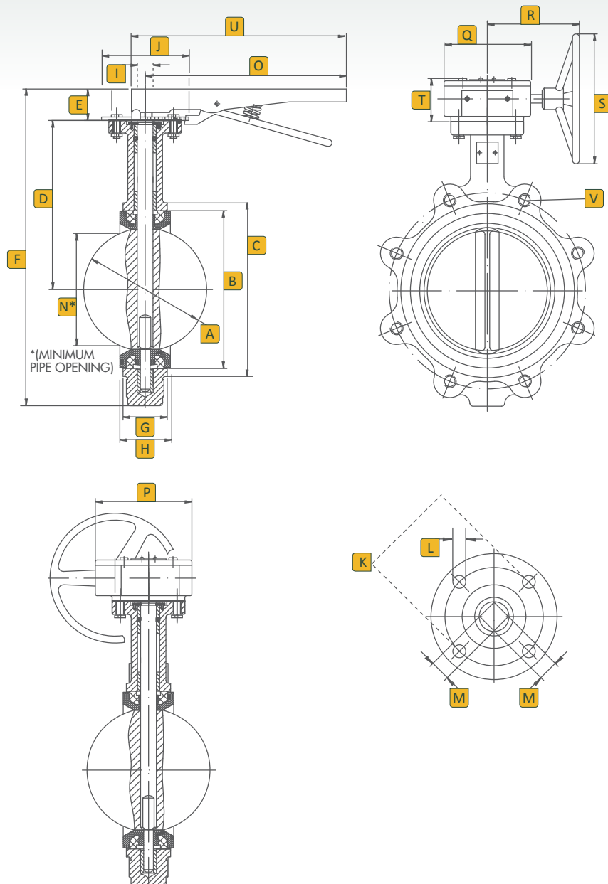
Dimensions (Inches)
