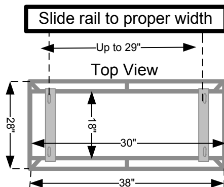
Mini Split Stand (gray) 18" High Part # MIN1832T Pad Size: 38 x 44"
