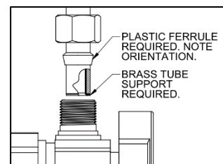
Figure 2: Supply Valve Connection
