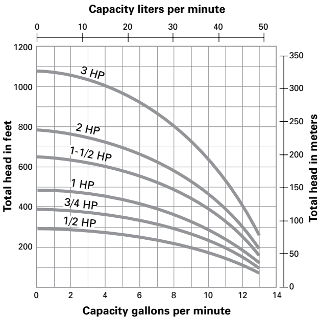
PUMP PERFORMANCE – 8 GPM
