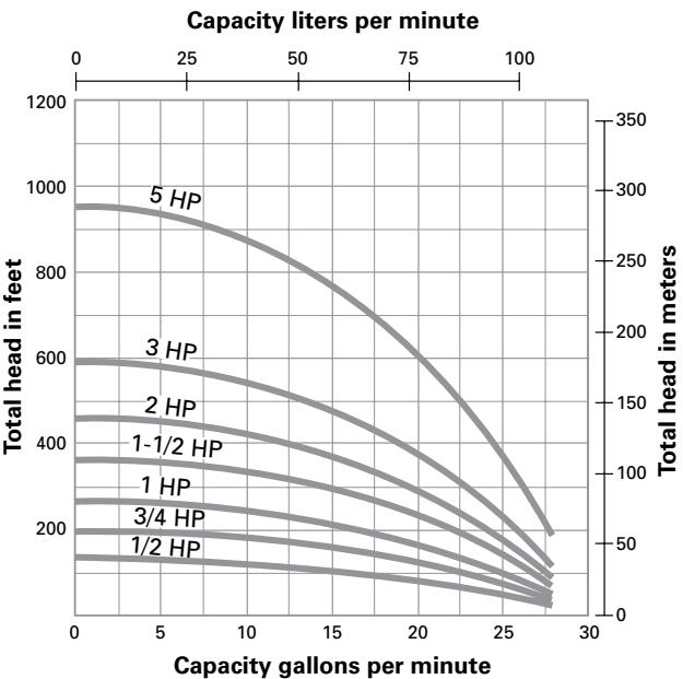
PUMP PERFORMANCE – 20 GPM
