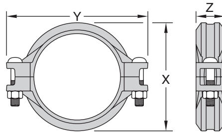
FIGURE 7401SS STAINLESS STEEL RIGID COUPLING
