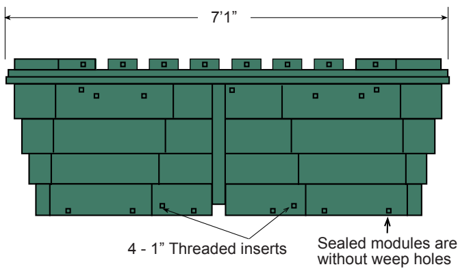
Elevation View
