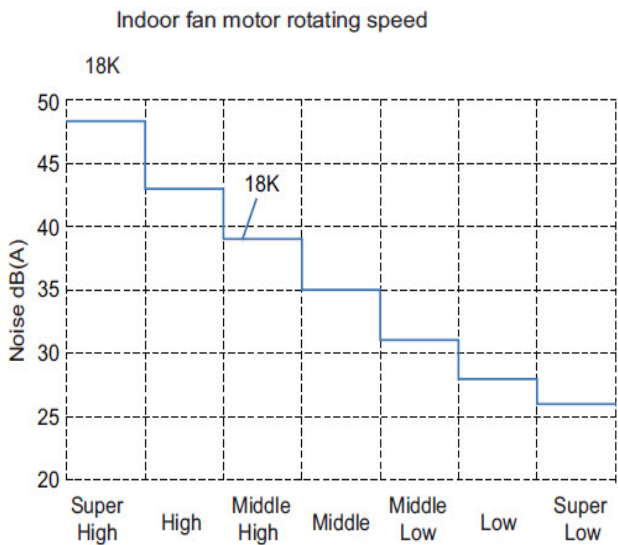
Fig. 10 – Sound curve
