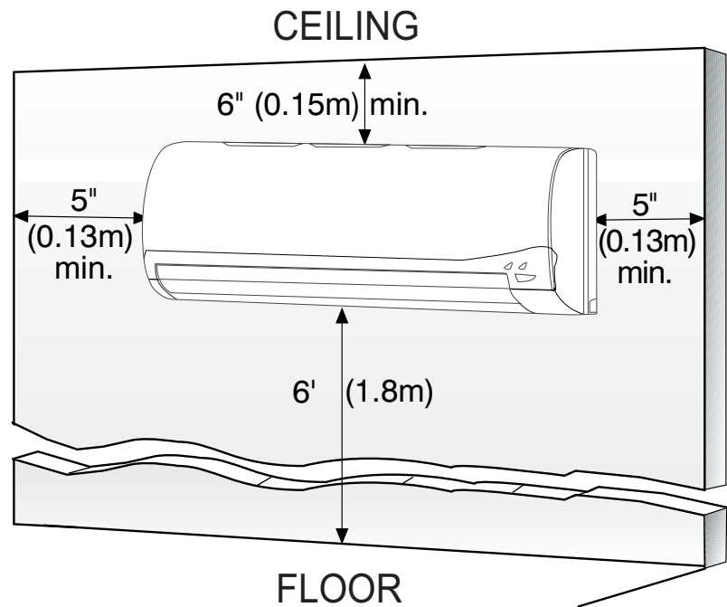
Fig. 5 – Indoor Unit Clearance
