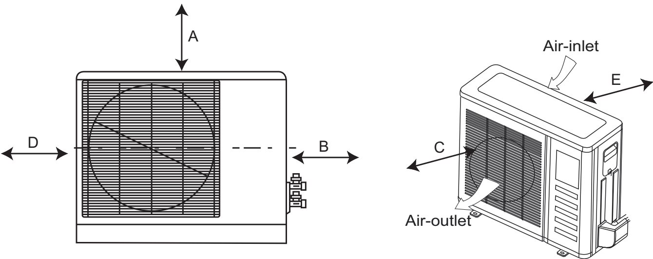
Fig. 6 – Clearances Outdoor
