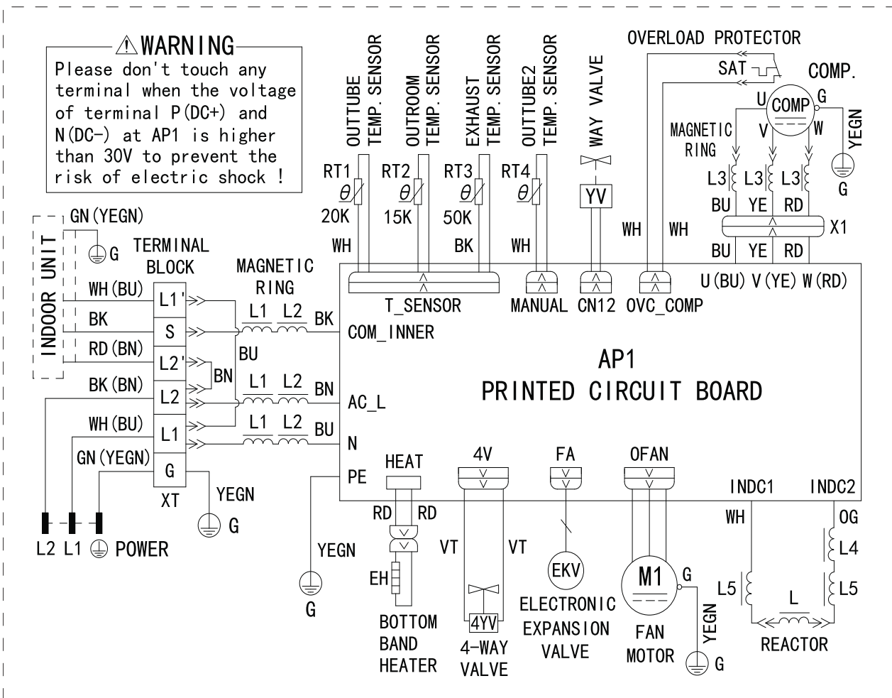
Fig. 15 – Outdoor Unit
