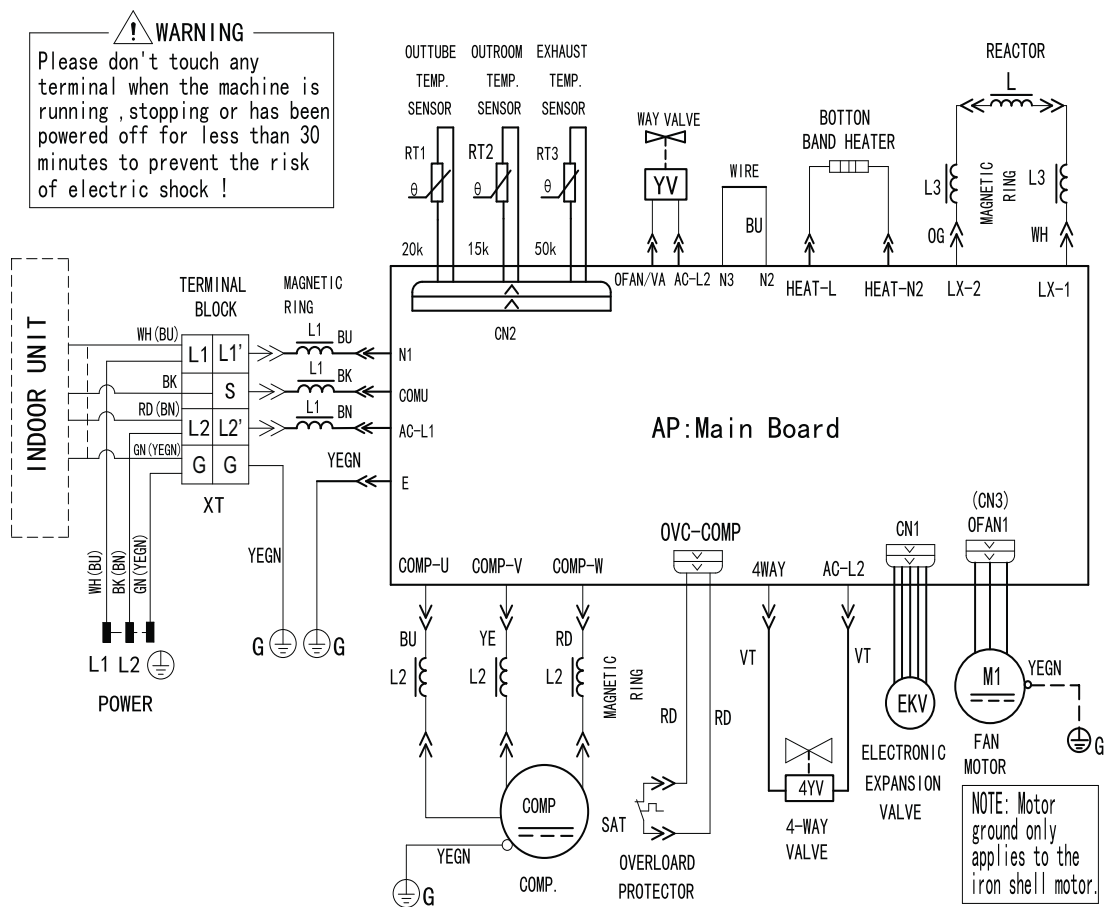
Fig. 14 – Outdoor Unit
