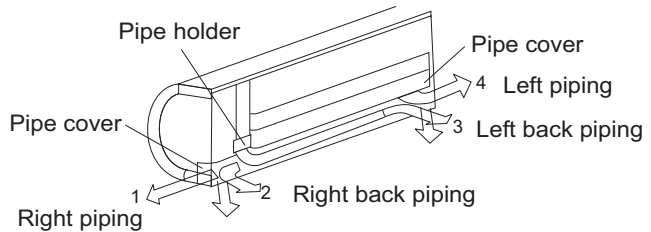
Fig. 11 – Piping Locations
