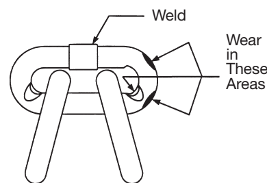
Figure 5a - Chain Inspection
