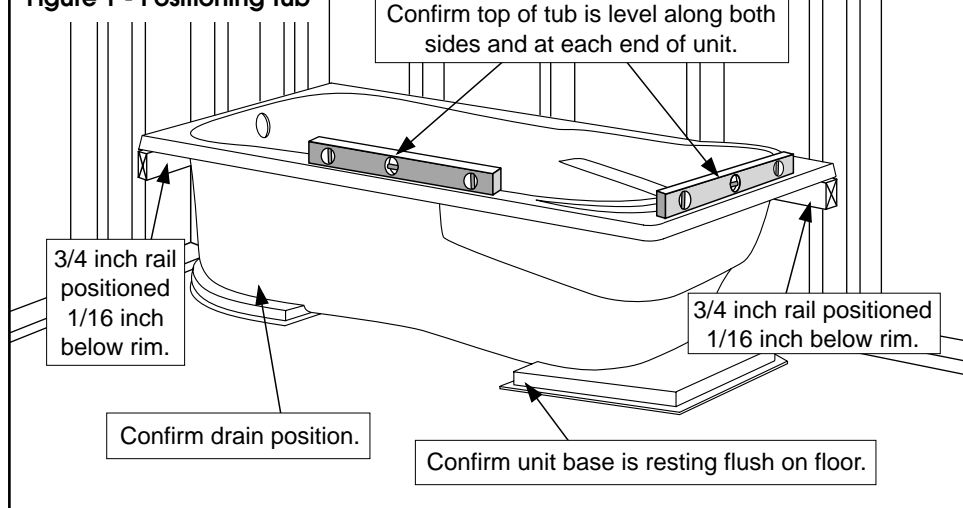
Figure 1 - Positioning Tub
