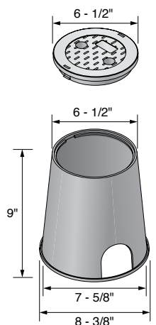
2-3/4" x 2-3/8" Pipe Slot
