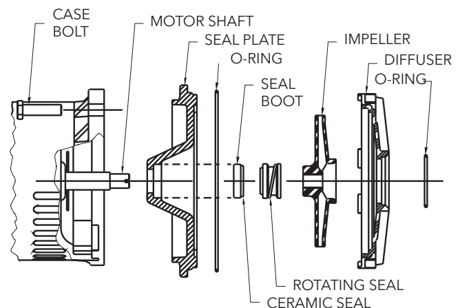
Figure 3: Seal assembly.
