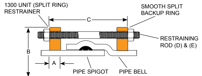
1355 ASSEMBLY
