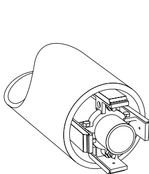
CASING SPACER FOR SUPPORT OF PIPE BARREL
