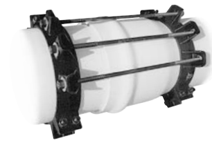
14" - 42" Series 1390 Installed
