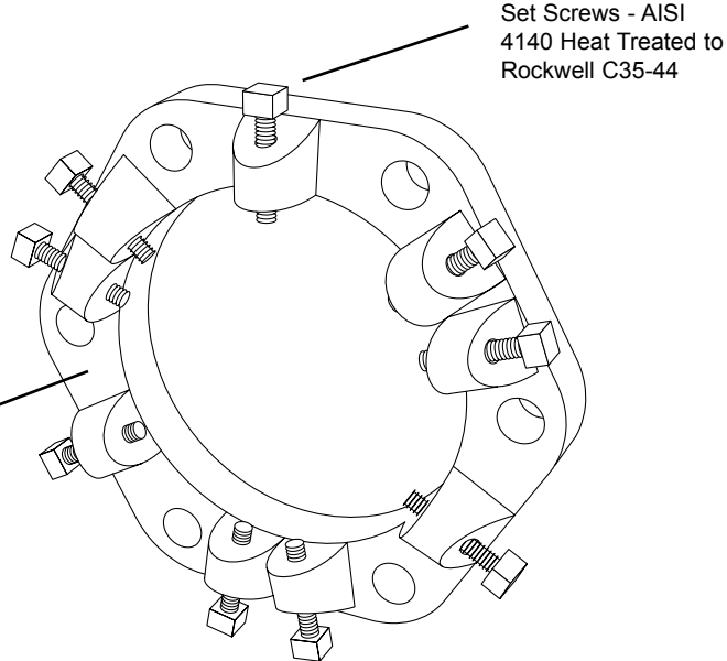
8" Model B
