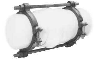
4" - 12" Series 1355 Installed
