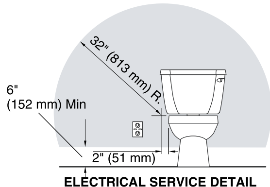
ELECTRICAL SERVICE DETAIL
