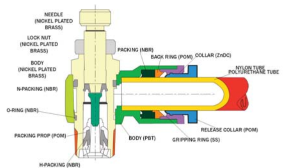
Figure 1.4 Diagram of Flow Controller
