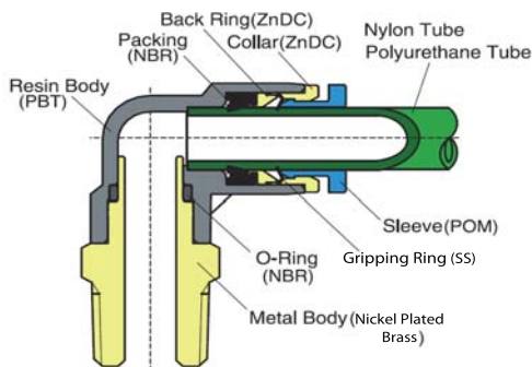
Figure 1.3 Diagram of Thread Fittings
